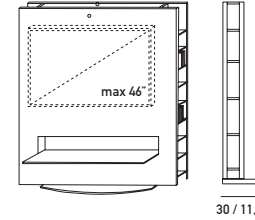
art. HF3 Base. Base L/W 105 P/D 30 W 41.3" D 11.8"
