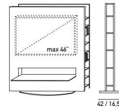
art. HF2 Base. Base L/W 105 P/D 42 W 41.3" D 16.5" Pannello. Unit. L/W 144 H 160 P/D 14 W 56.7" H 63" D 5.5"
