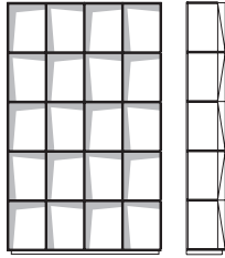
C2 L/W 124 H 184.2 P/D 31 W 48.8" H 72.5" D 12.2"
