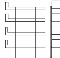
Art. 9100 DX - Art. 9100 SX L/W 165 H 188 P/D 40 SX/DX W 65" H 74" D 15.7" (left or right)
